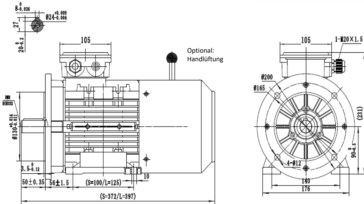
Typ / type SEV-BM3 90S-8
